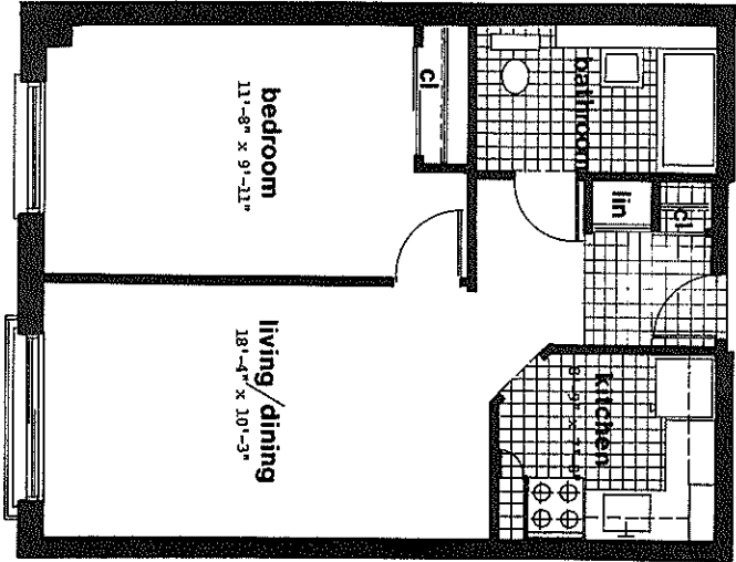
ONE BEDROOM HANDICAPPED UNIT (1B-3H)
