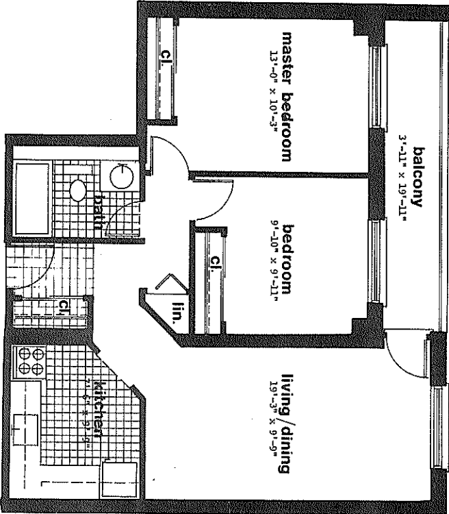
TWO BEDROOM UNIT (2B-2)
