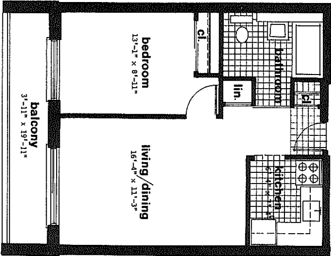
ONE BEDROOM HANDICAPPED UNIT (1B-4H)
