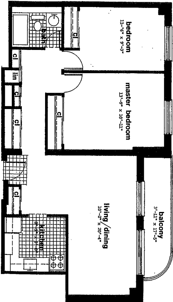
TWO BEDROOM UNIT (2B-7)
