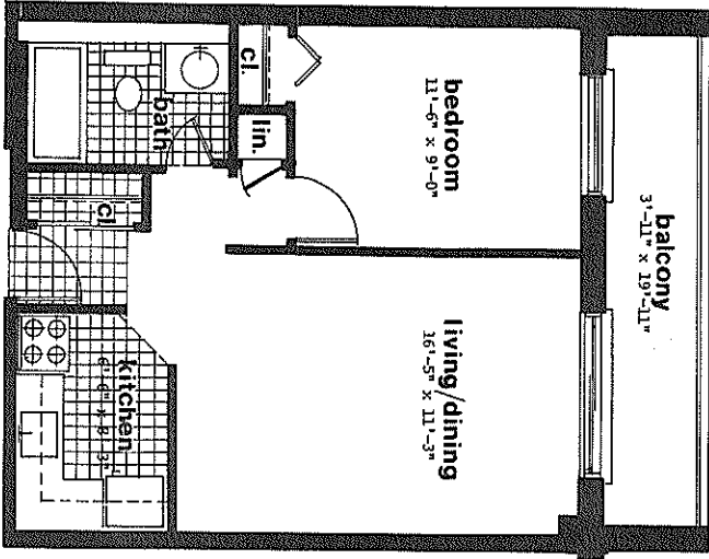
ONE BEDROOM UNIT (1B-2)
